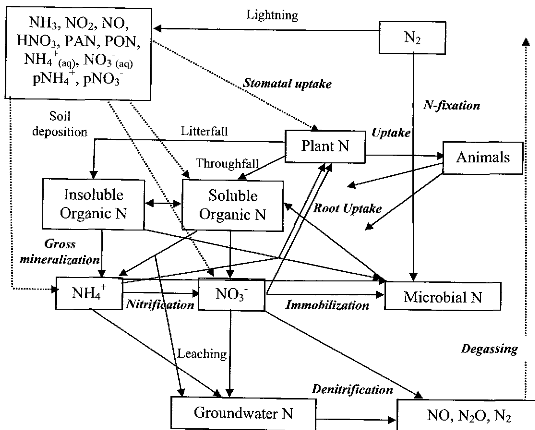
Figure 1. The N-cycle simplified. Biological processes are labeled in bold italics, and the lighter arrows show deposition pathways.
