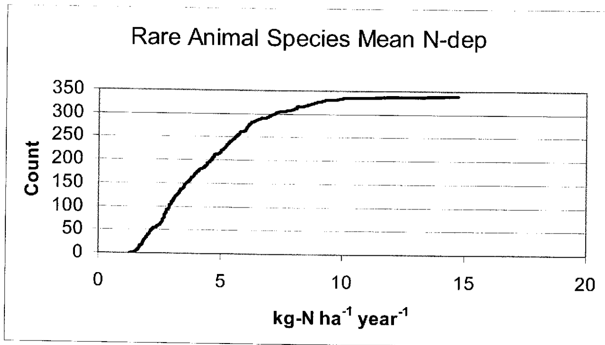
Figure 20. Mean N-deposition exposure, state- and federal-listed rare animal taxa (n = 339)
