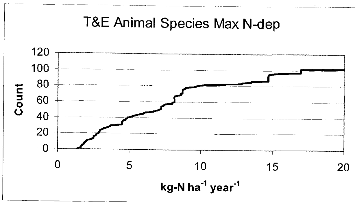
Figure 19. Maximum N-deposition exposure, state- and federal-listed T&E animal taxa (n = 108)
