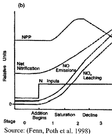
Figure 2. Stages of N-saturation in western xeric forests
