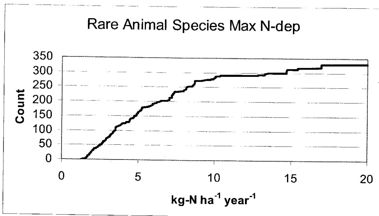
Figure 21. Maximum N-deposition exposure, state- and federal-listed rare animal taxa (n = 339)
