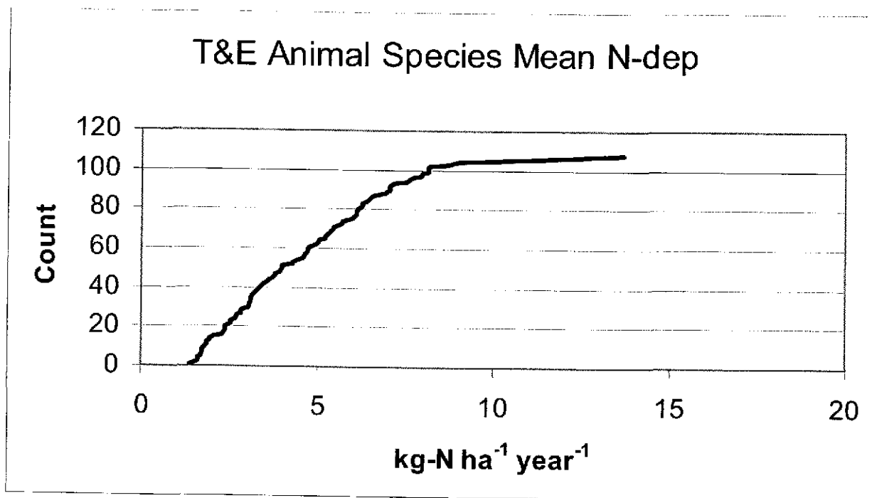
Figure 18. Average N-deposition exposure, state- and federal-listed T&E animal taxa (n = 108)
