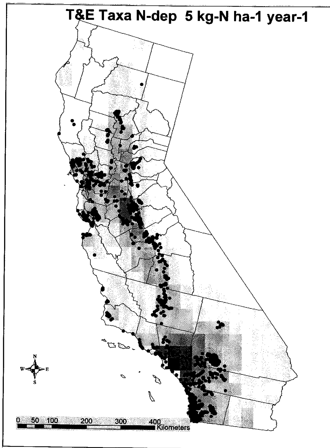
Figure 15. Distribution of federal- and state-listed T&E species exposed to > 5 kg-N ha -1 year -1
