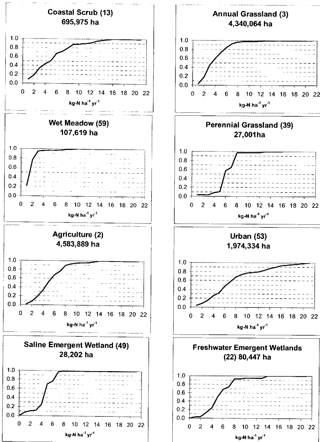
Figure 10. Cumulative distribution functions of N-deposition exposure of FRAP vegetation types. The FRAP code numbers for each vegetation type are in parentheses, followed by total area in hectares so that proportions (Y axis) may be converted to area affected. Maps of each vegetation type are presented in Appendix A, in the same order.
