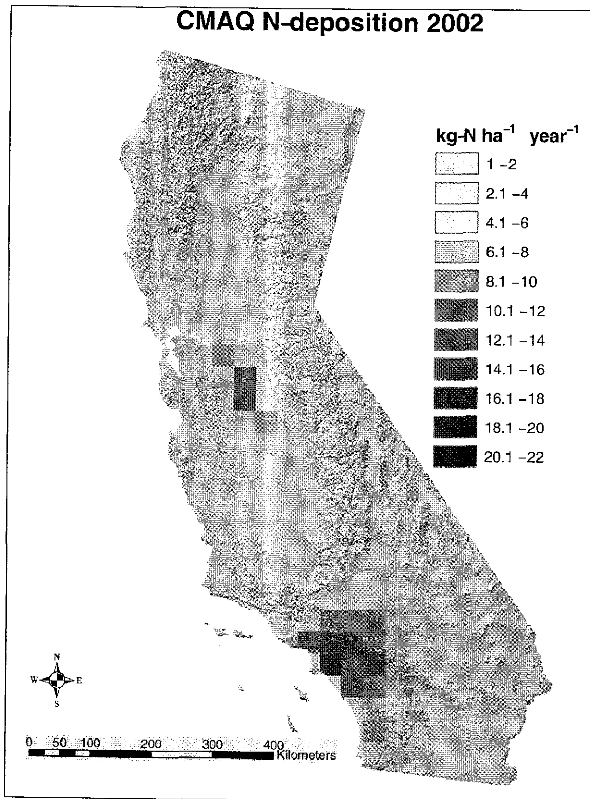
Figure 7. CMAQ 36 km N-deposition
