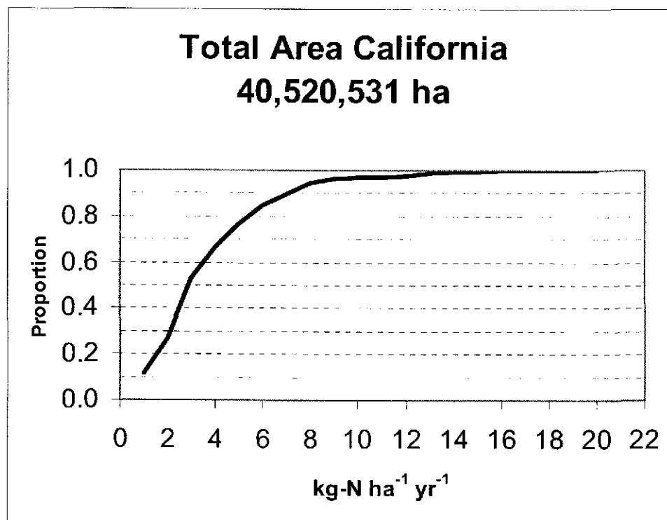
Figure 8. Statewide N-deposition proportion (CDF format)
